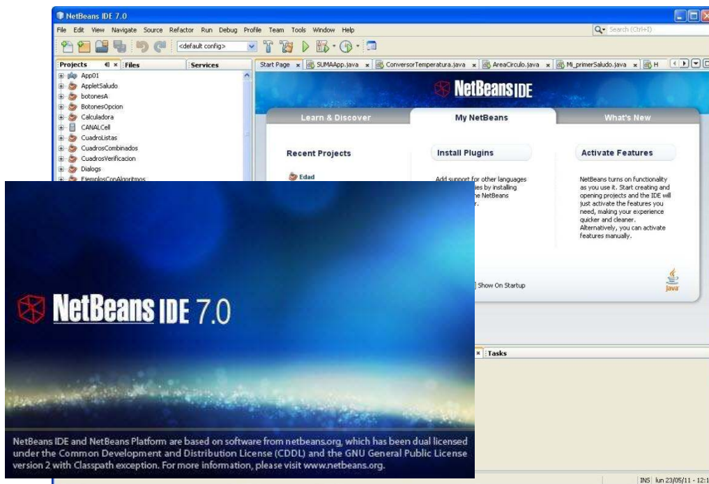
Figura 5 IDE NetBeans 7.0
